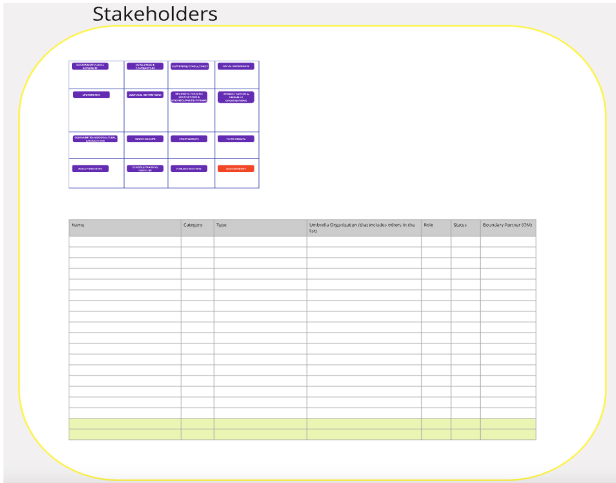
Fig. 1 – stakeholder mapping
