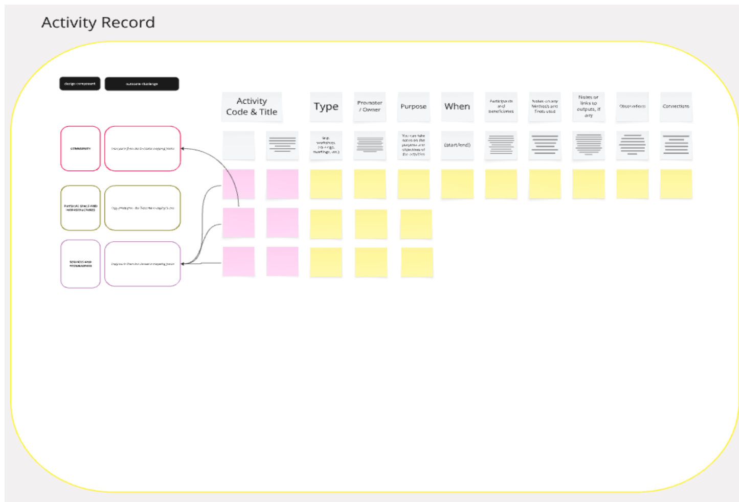
Fig 3 – Activity record
