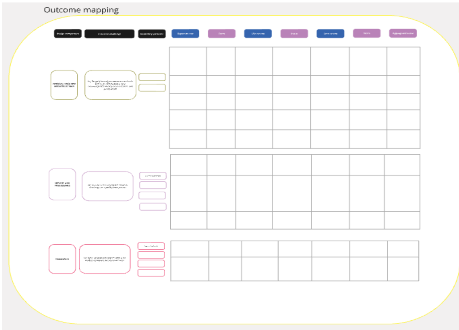
Fig 2 – Outcome mapping
